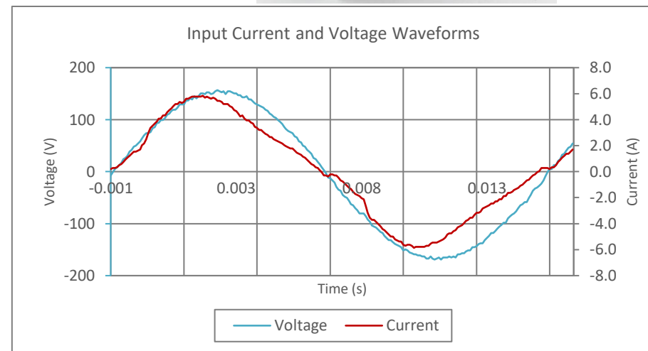
Input AC Current Waveform (ITHD = 14.82%, 50% Load)
