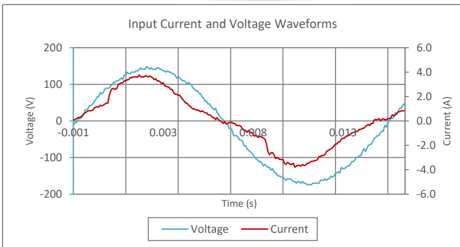
Input AC Current Waveform (ITHD = 21.38%, 50% Load)
